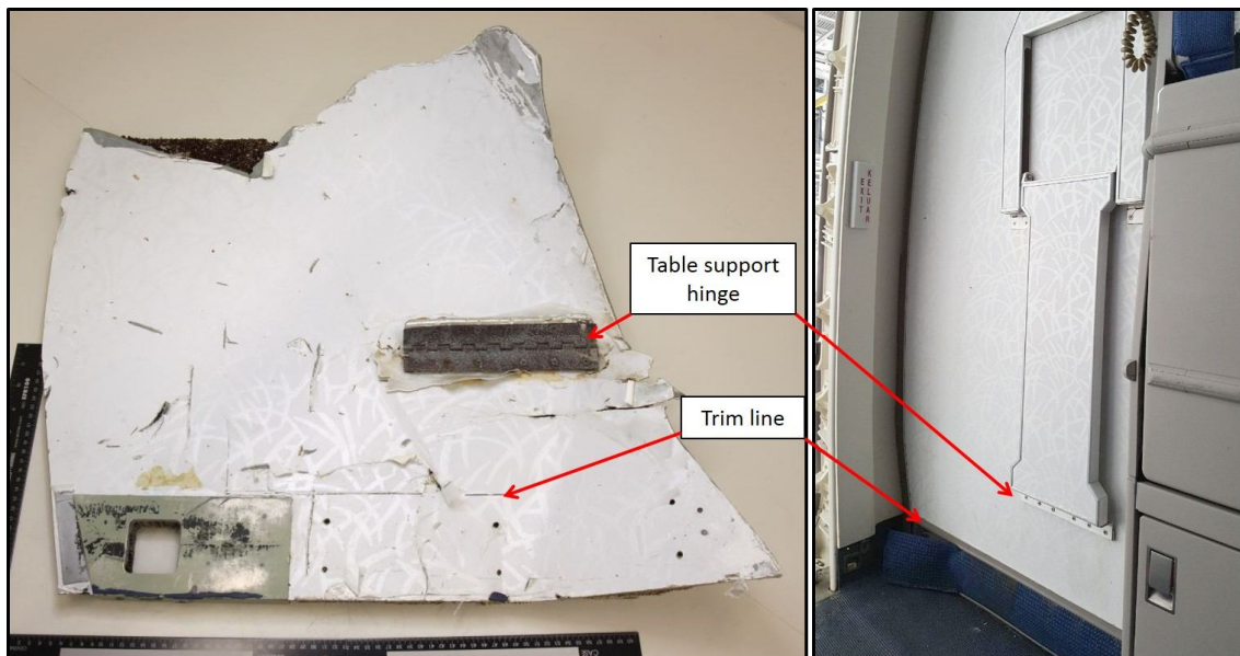
Figure 2: Comparison of recovered item with MAB Boeing 777 Door R1 panel assembly
